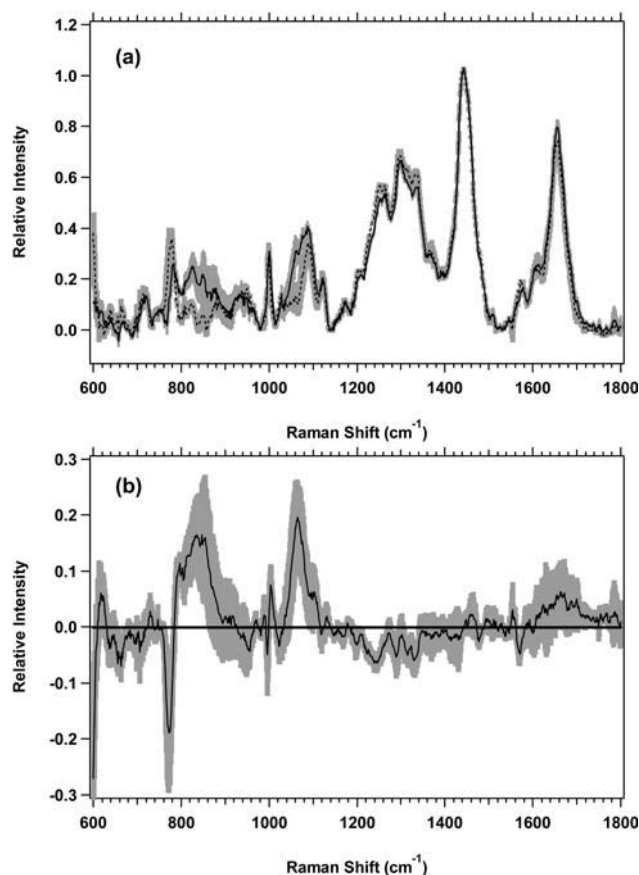
FIGURE 6 (a) Standard deviations (shaded area) overlying the averages are shown from 600 to 1800 cm -1 for M1 plateau (solid line) ( n = 3 ) and exponential (dotted line) ( n = 3 ) nuclei. The spectra have been normalized to the integrated intensity from 1437 to 1453 cm -1 . (b) Difference spectrum for M1 plateau minus M1 exponential nuclei, with its standard deviation, is shown.
