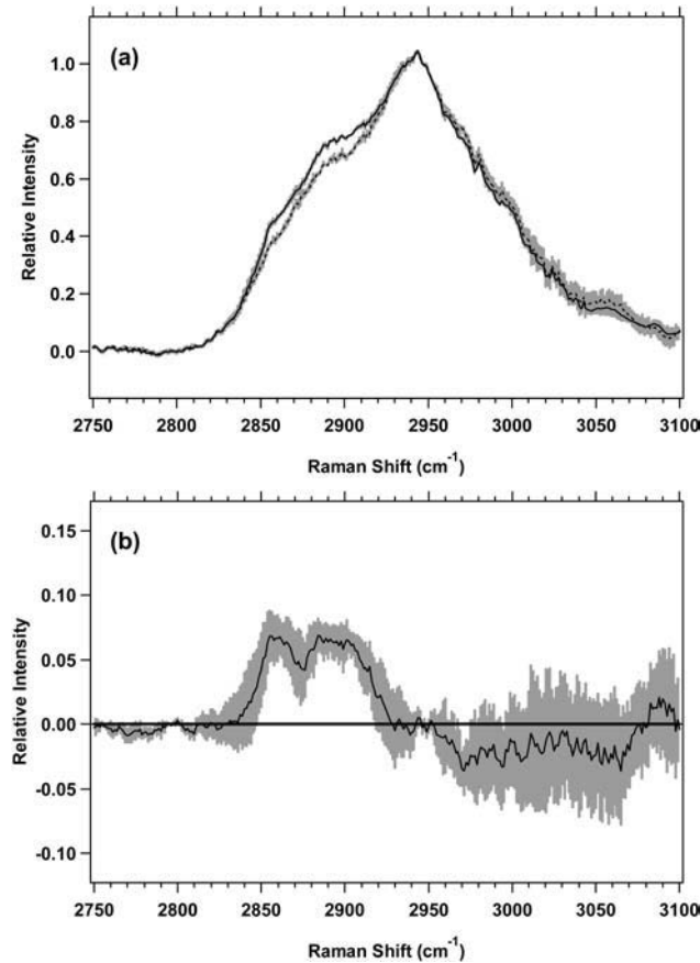
FIGURE 4 (a) Standard deviations (shaded area) overlying the averages are shown from 2750 to 3100 \text{cm}^{-1} for M1 plateau (solid line) ( n = 7 ) and exponential (dotted line) ( n = 7 ) cells. The spectra have been normalized to the integrated intensity from 2929 to 2940 \text{cm}^{-1} . (b) Difference spectrum for M1 plateau minus M1 exponential cells, with its standard deviation, is shown.
