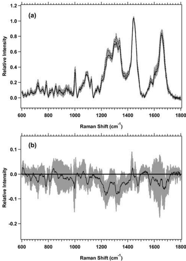
FIGURE 3 (a) Standard deviations (shaded area) overlying the averages are shown from 600 to 1800 \text{cm}^{-1} for MR1 plateau (solid line) ( n = 8 ) and exponential (dotted line) ( n = 7 ) cells. The spectra have been normalized to the integrated intensity from 1437 to 1453 \text{cm}^{-1} . (b) Difference spectrum for the averages of MR1 plateau minus MR1 exponential cells, with its standard deviation, is shown.
