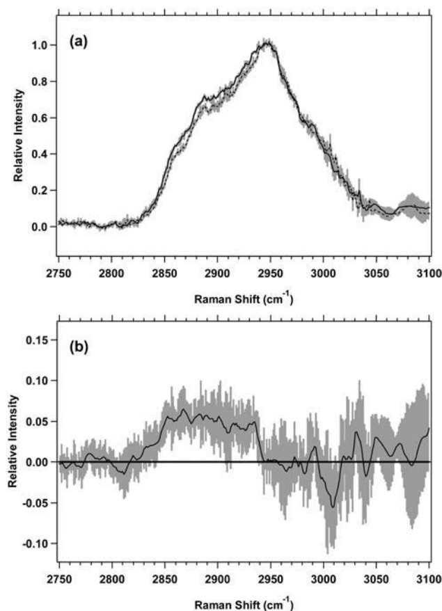
FIGURE 5 (a) Standard deviations (shaded area) overlying the averages are shown from 2750 to 3100 cm -1 for MR1 plateau (solid line) ( n = 7 ) and exponential (dotted line) ( n = 7 ) cells. The spectra have been normalized to the integrated intensity from 2929 to 2940 cm -1 . (b) Difference spectrum for MR1 plateau minus MR1 exponential cells, with its standard deviation, is shown.
